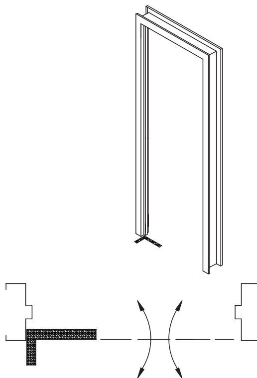
FIGURE 12 FRAME TWIST CHECK
